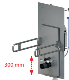
AM101/1500L Medic Assistant Pre-wall installation system for dry build up, height adjustable – for people with reduced mobility
